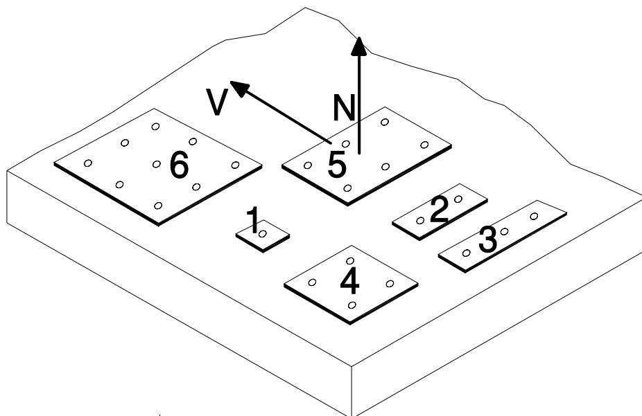
Figure 16: Types of anchor plates approved by European Technical Approvals (ETA)
